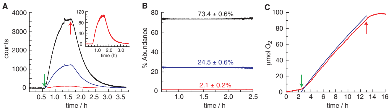
Fig. 3. (A) Mass spectrometric detection of isotopically labeled ^{16,16}\text{O}_2 (black line), ^{16,18}\text{O}_2 (blue line), and ^{18,18}\text{O}_2 (red line) during electrolysis of a catalyst film on ITO in a KPi electrolyte containing 14.6% ^{18}\text{OH}_2 . The green arrow indicates the initiation of electrolysis at 1.29 V (NHE), and the red arrow indicates the termination of electrolysis. (Inset) Expansion of the ^{18,18}\text{O}_2 signal. (B) Percent abundance of each isotope over the course of the
