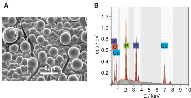
Fig. 2. (A) SEM image ( 30^\circ tilt) of the electrodeposited catalyst after 30 C/cm 2 were passed in 0.1 M KPi electrolyte at pH 7.0, containing 0.5 mM \text{Co}^{2+} . The ITO substrate can be seen through cracks in the dried film. (B) Typical EDX histogram acquired at 12 kV. cps, counts per second.
